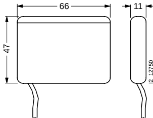
7LF4 940-0 Card reader for USB connection
