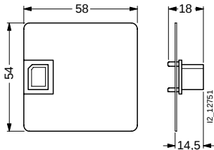
Insert card for data key
