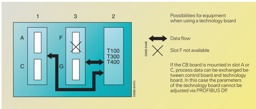
Fig. 6/60 Integration of boards in the electronics box
