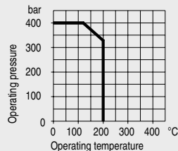
Fig. 1/84 Permissible operating pressure
