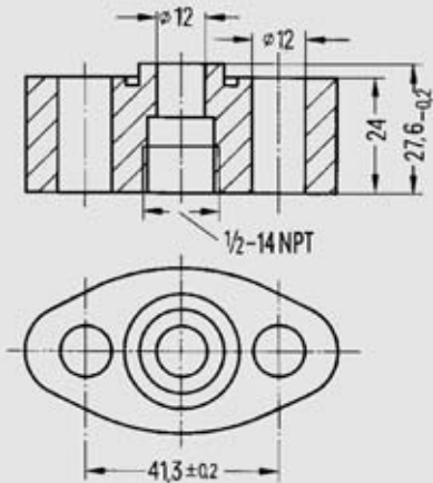
Fig. 1/124 Oval flange, dimensions
