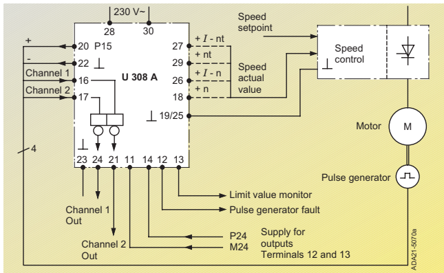
Fig. 3/4 Block diagram
