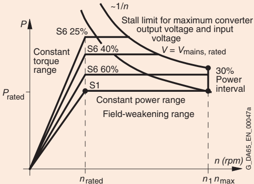
Power-Speed Curve
